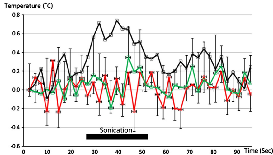
Fig. 7. Tissue temperature measured using MR thermometry from the sonication locus (red line) and the control non-sonicated site (green line) ( n = 7 ; shown with standard error). The sonication duration is shown by a black bar. The black solid line indicates that a slight temperature rise (less than 0.8^{\circ}\text{C} ) was detected when higher acoustic intensity ( I_{\text{sppa}} = 23 \text{ W/cm}^2 ) was given at the same pulsing scheme (i.e., \text{TBD} = 0.5 \text{ msec} and \text{PRF} = 100 \text{ Hz} ; I_{\text{spta}} = 1.15 \text{ W/cm}^2 ).
